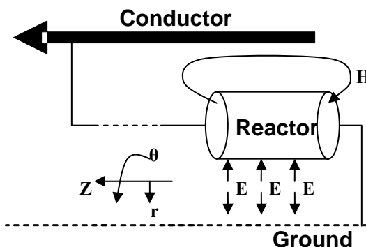
Fig. 3 Shunt reactor showing coordinate system and location of electric and magnetic fields
