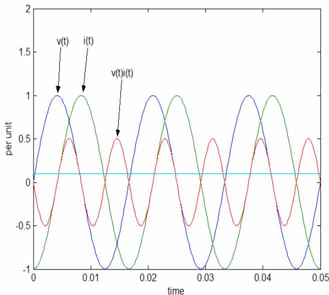
Fig. 4 Instantaneous voltage and current in a reactor. The instantaneous power is p(t) = v(t)i(t) .
