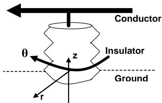
Fig. 2 Post-type insulator showing coordinate system
